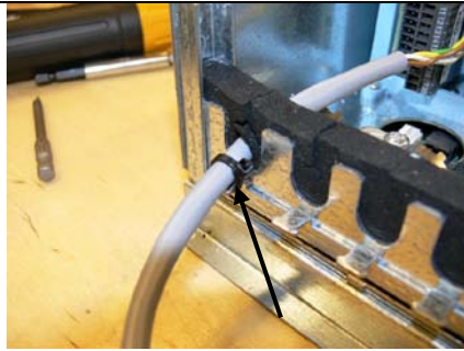
11. Attach the cable to the washer with a plastic binder
